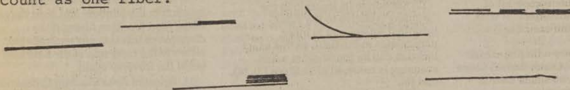
Figure 1.—Counting guidelines used in determining asbestos structures. (From Yamate et al., 1984)
