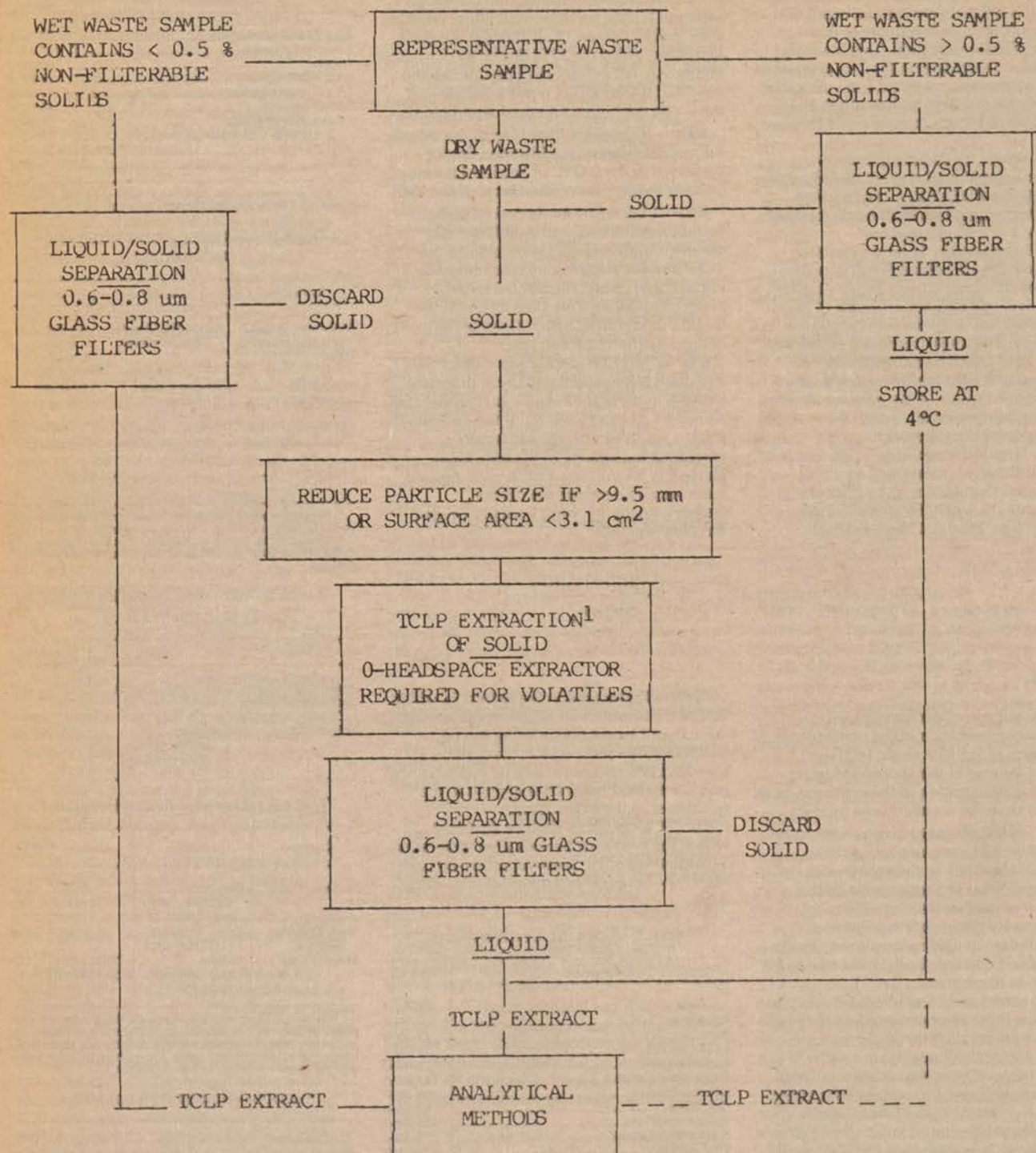
FIGURE 1: TCLP Flowchart
