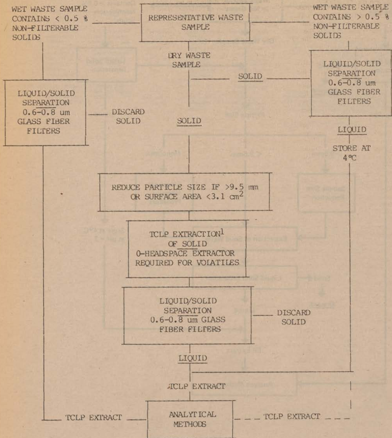
FIGURE D-2: TCLP Flowchart
